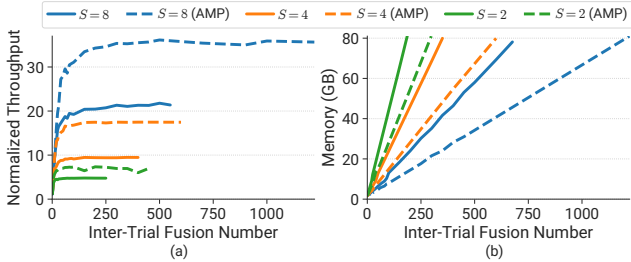
Figure 13: Sensitivity analysis of S and AMP on ResNet-18. (a) Accumulated throughput. (b) GPU memory footprint.
